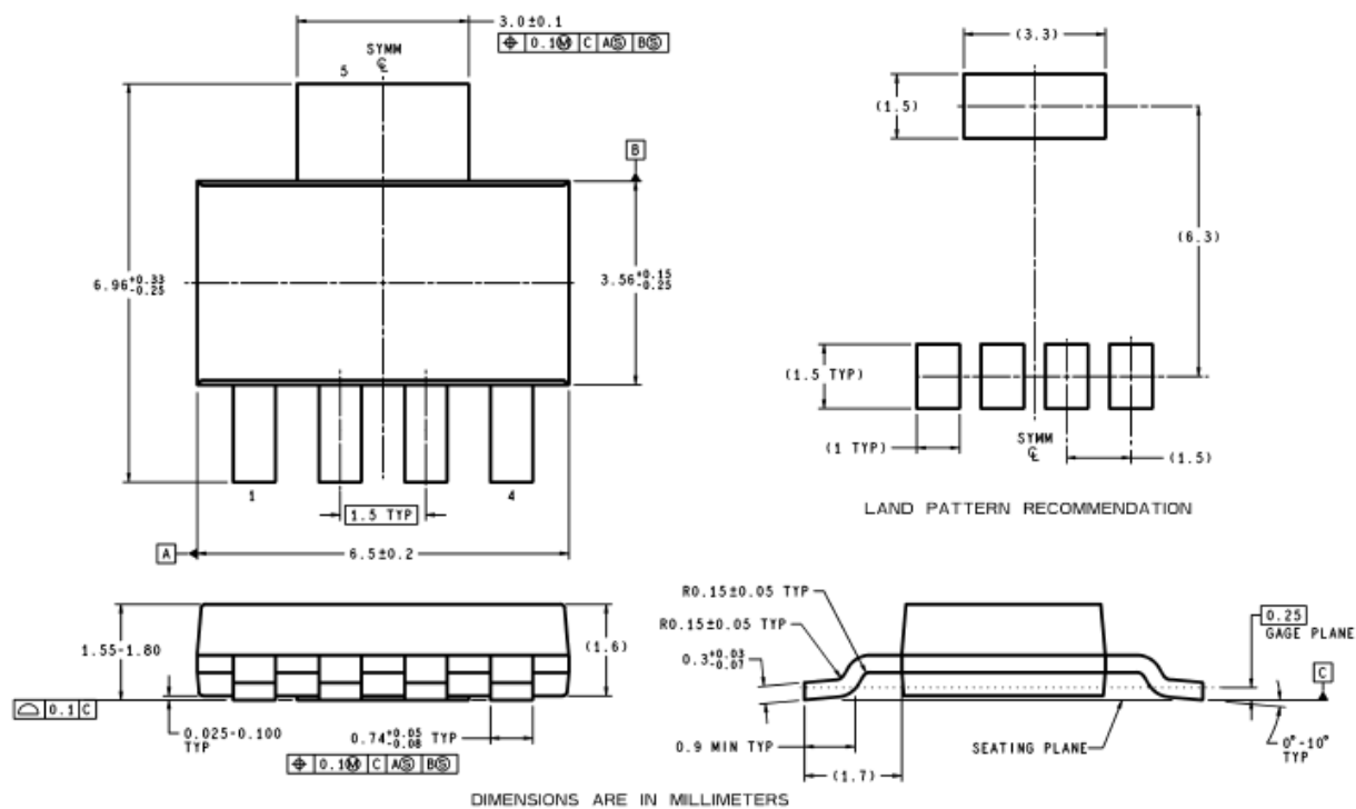
SOT223, 5-Lead, Molded, Surface Mount Package (SOT223-5)
