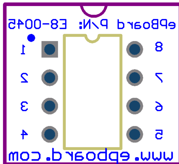
Bottom Side (Top View X-Ray)
