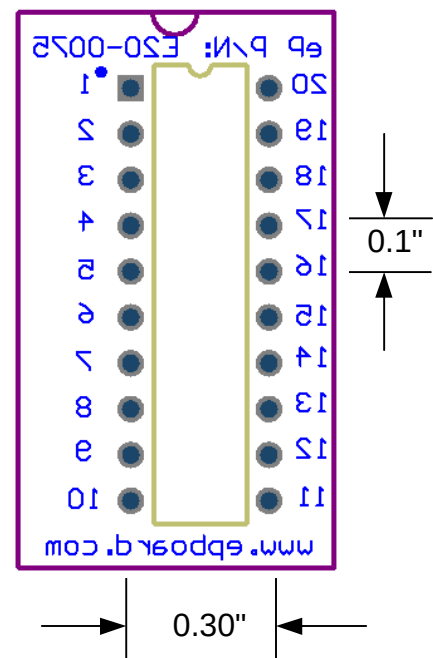
Bottom Side (Top View X-Ray)
