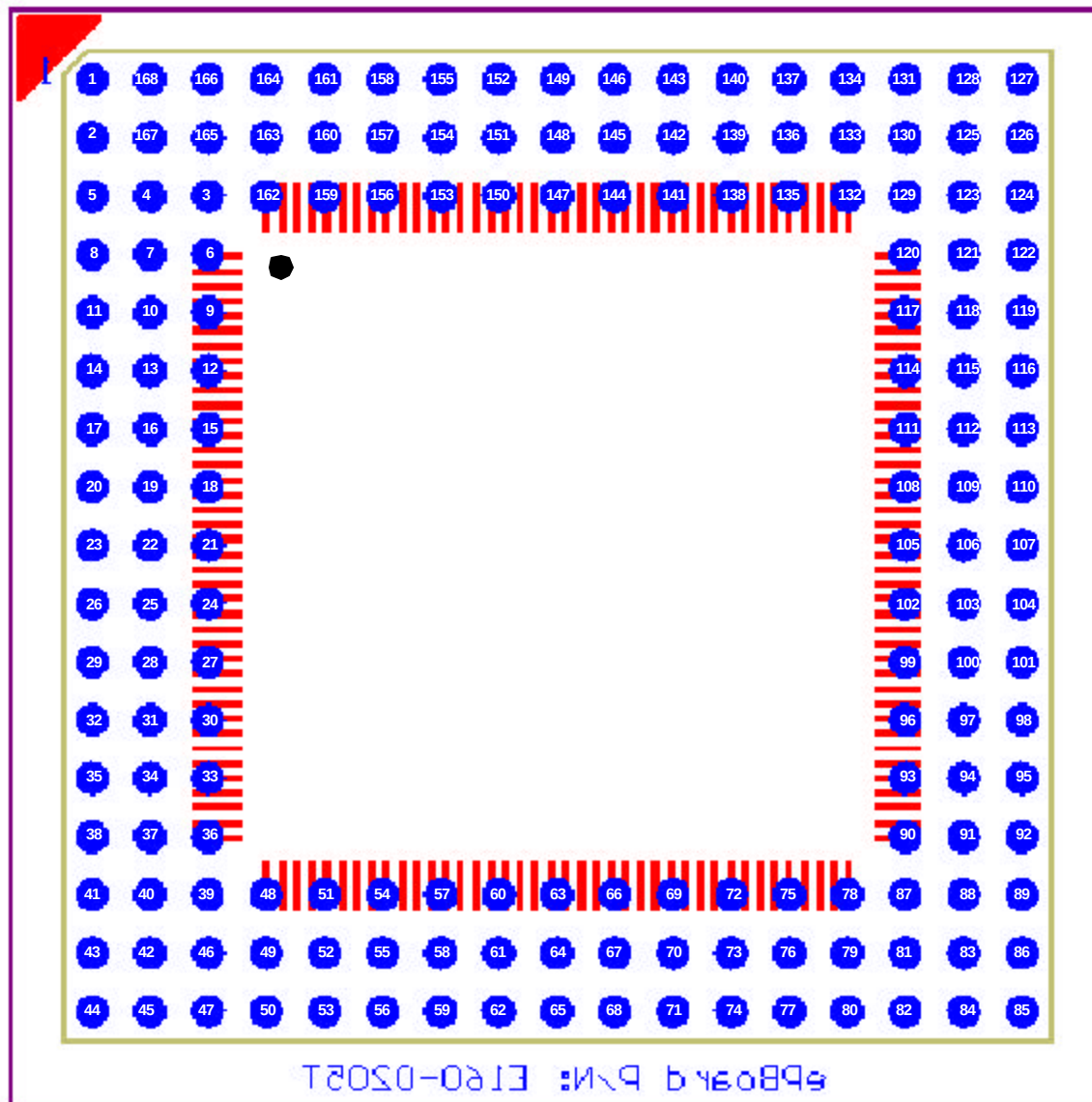
Top View X-Ray with PGA pin assignment
