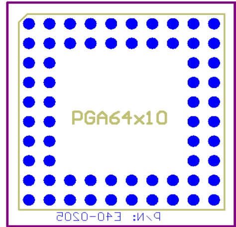
Mill-Max PGA Socket (510-93-064-10-051)
