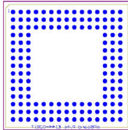
Mill-Max PGA Socket (510-93-144-15-082001)
